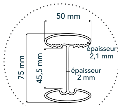
POTEAU ATOLL +
