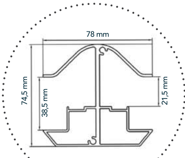
POTEAU OASIS
