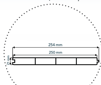
LAME OASIS 250
