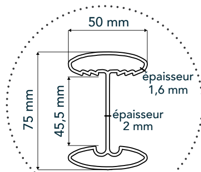
POTEAU ATOLL
