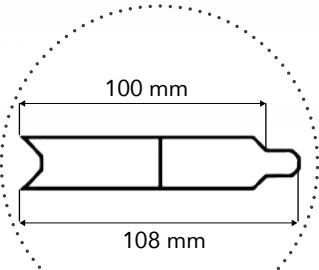
LAME OCEAN
