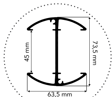
POTEAU LAME BOIS
