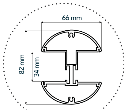
POTEAU ALUMINIUM ARCHIPEL
