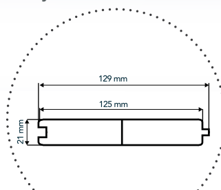
LAME OASIS 125
